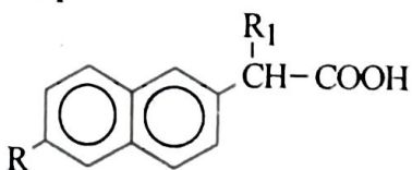
Scheme 16.11
