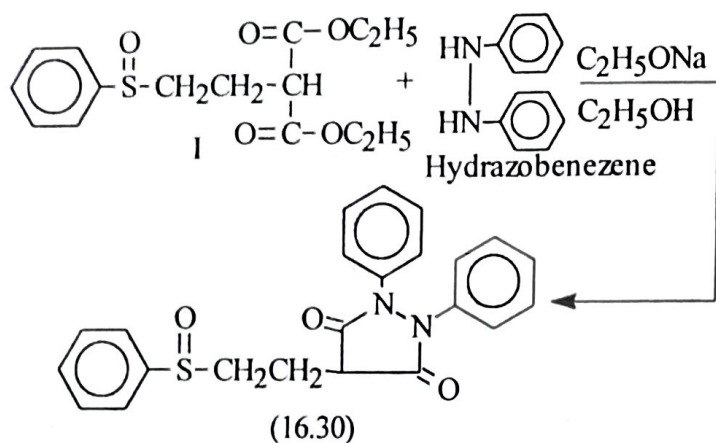
Scheme 16.28
