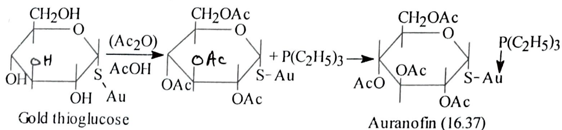
Scheme 16.20
